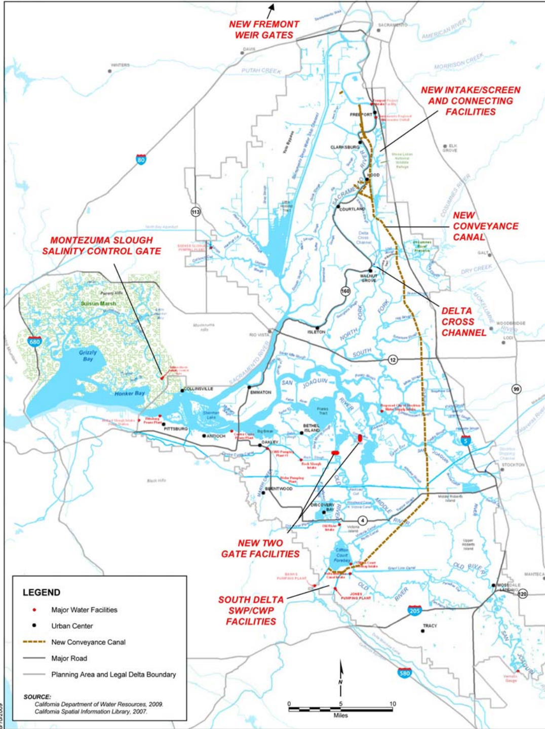
6/18/09 DRAFT Location of New Conveyance and Intake Facilities
